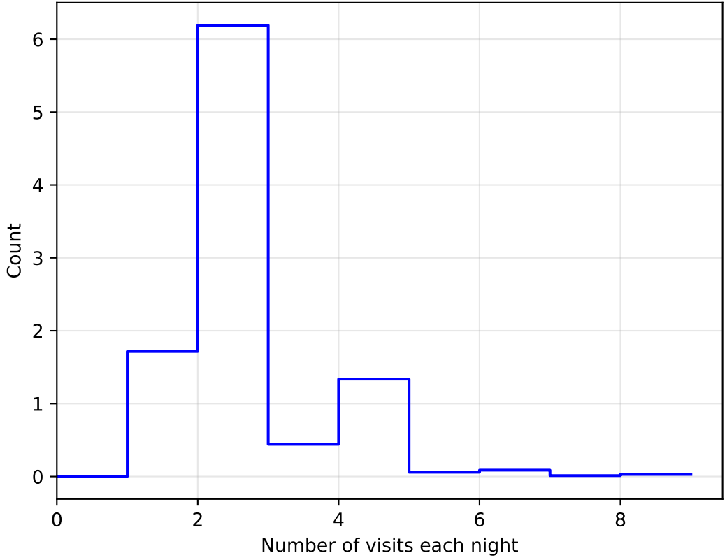
ddf_acor_sf20_lsf40_lsr50_v3.4_10yrs All sky: NVisitsPerNight 1e6
