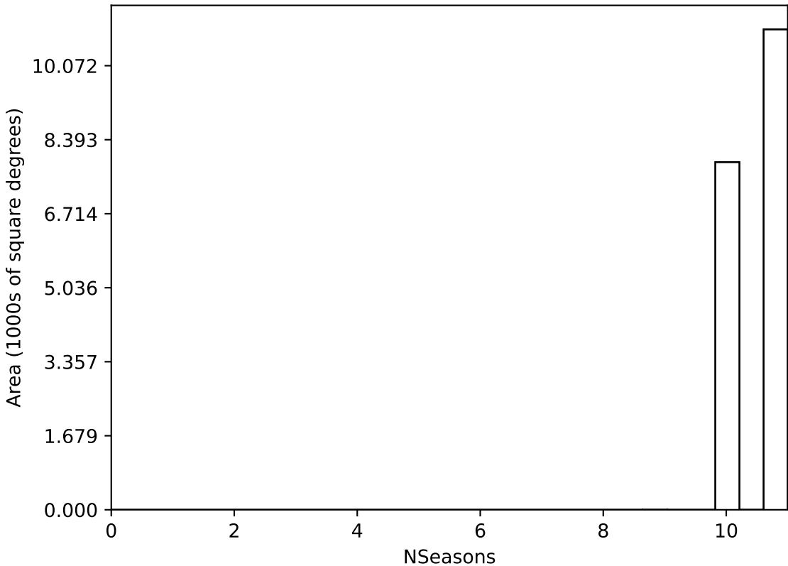
ddf_acor_sf20_lsf40_lsr50_v3.4_10yrs WFD all bands: NSeasons
