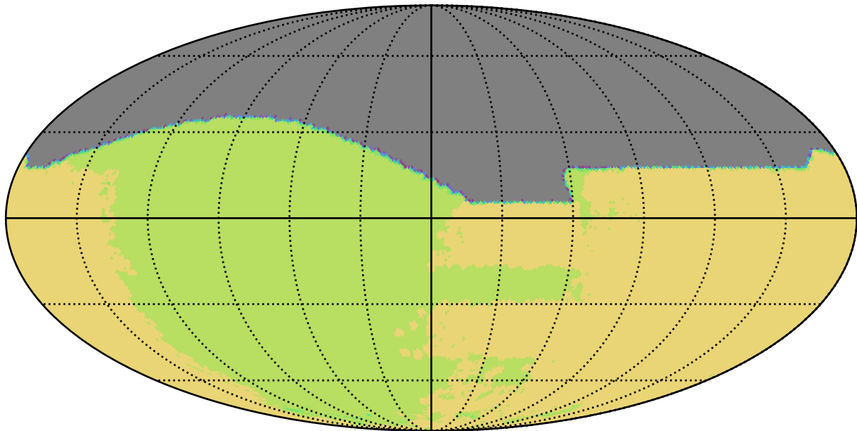
ddf_acor_sf20_lsf40_lsr50_v3.4_10yrs All sky all bands: NSeasons
