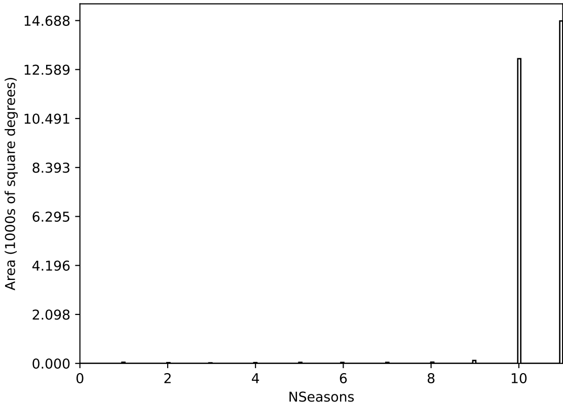
ddf_acor_sf20_lsf40_lsr50_v3.4_10yrs All sky all bands: NSeasons
