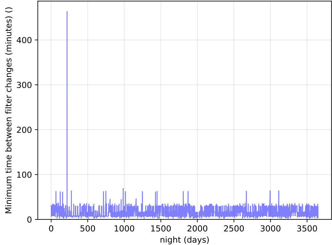
ddf_acor_sf20_Isf40_Isr50_v3.4_10yrs Per Night: Minimum time between filter changes (minutes)
