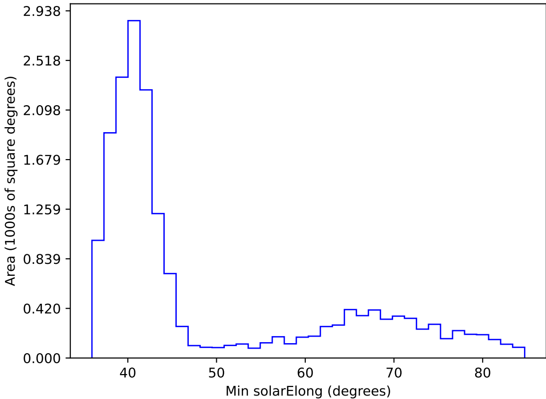
ddf_acor_sf20_lsf40_lsr50_v3.4_10yrs WFD z band: Min solarElong
