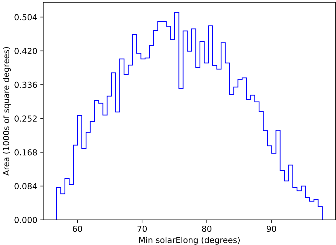
ddf_acor_sf20_lsf40_lsr50_v3.4_10yrs WFD u band: Min solarElong
