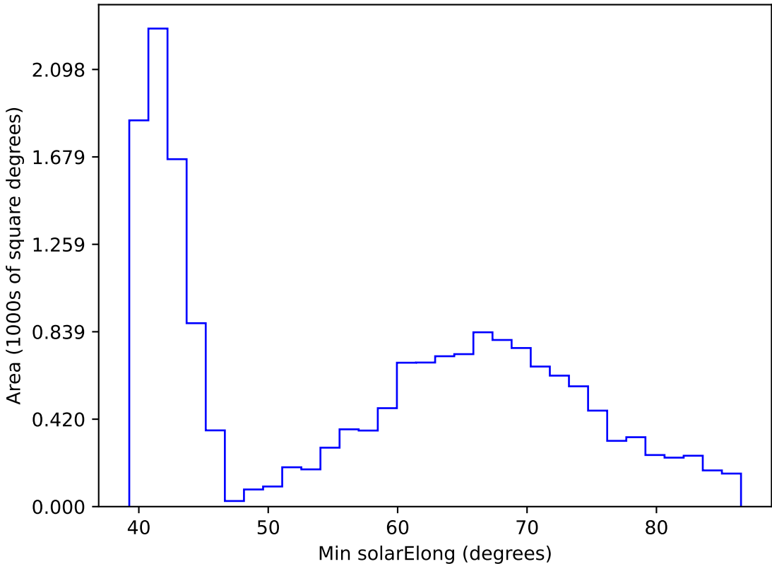
ddf_acor_sf20_lsf40_lsr50_v3.4_10yrs WFD r band: Min solarElong
