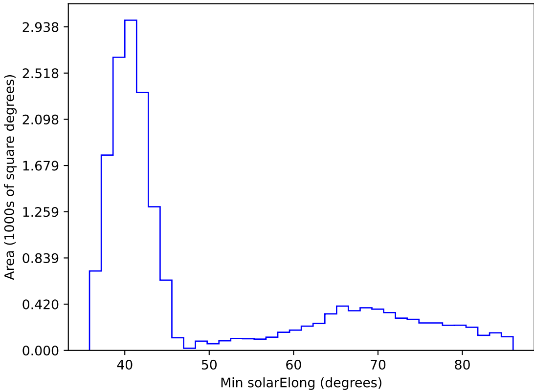
ddf_acor_sf20_lsf40_lsr50_v3.4_10yrs WFD i band: Min solarElong
