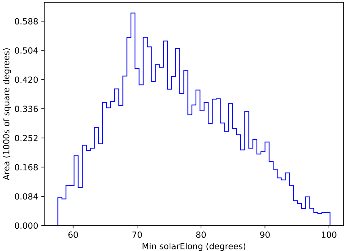
ddf_acor_sf20_lsf40_lsr50_v3.4_10yrs WFD g band: Min solarElong
