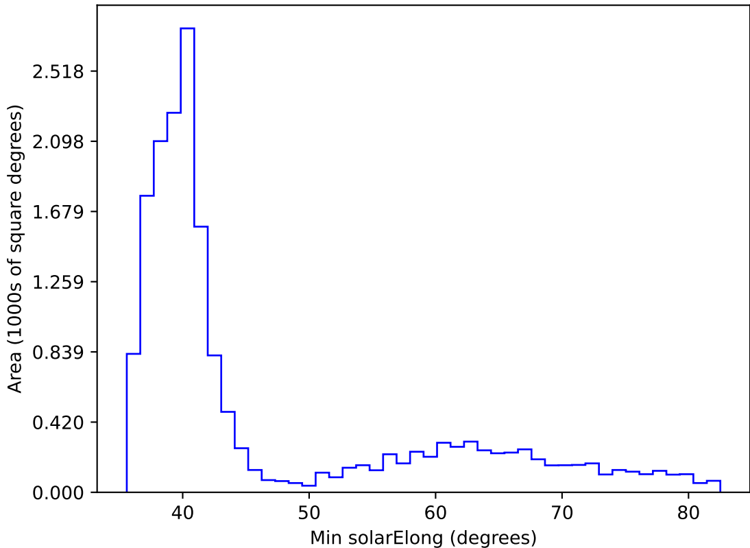
ddf_acor_sf20_lsf40_lsr50_v3.4_10yrs WFD all bands: Min solarElong
