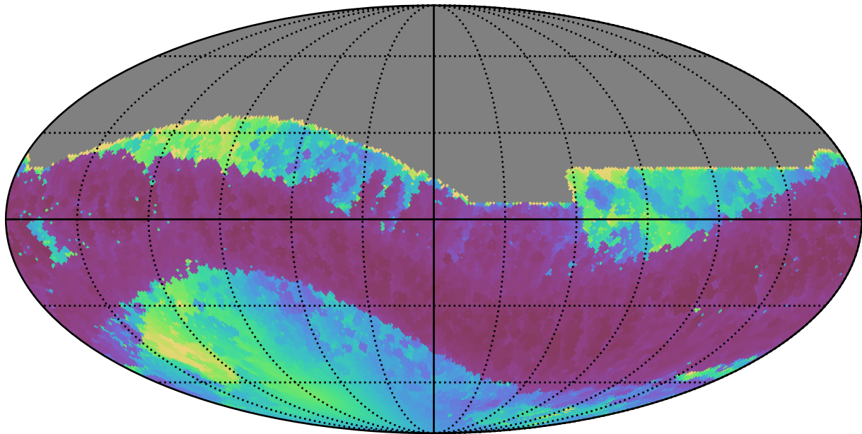
ddf_acor_sf20_lsf40_lsr50_v3.4_10yrs All sky z band: Min solarElong
