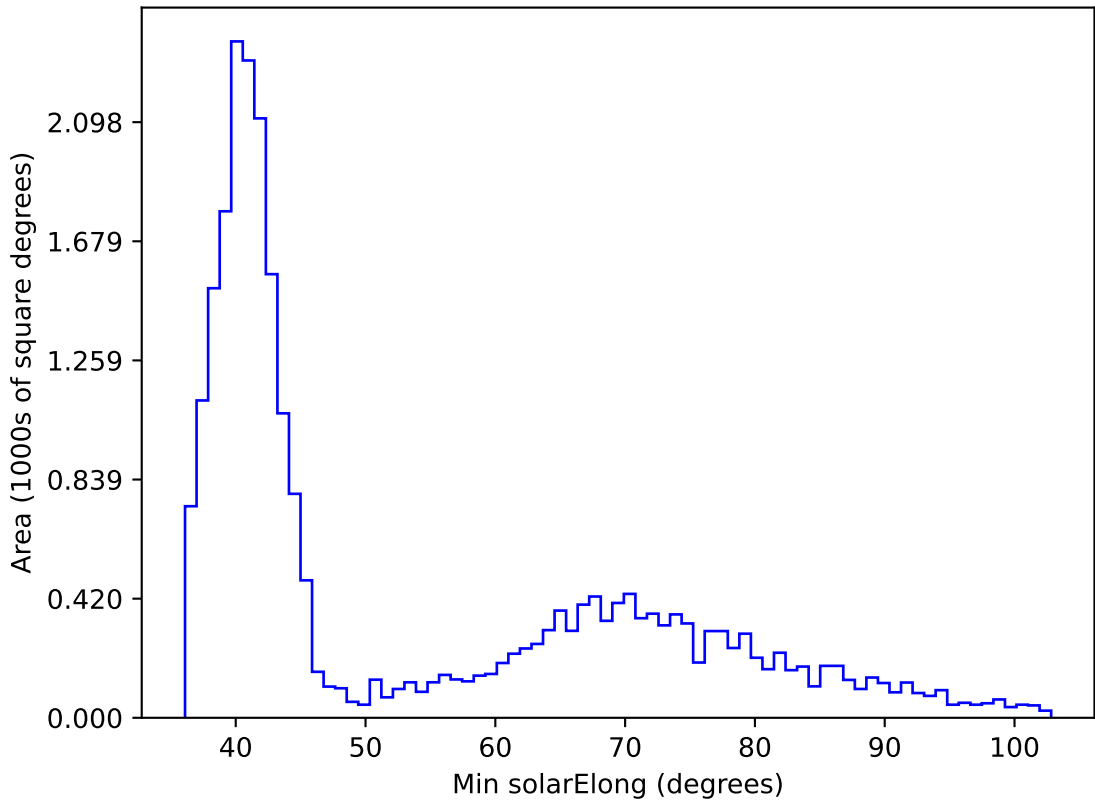
ddf_acor_sf20_lsf40_lsr50_v3.4_10yrs All sky z band: Min solarElong
