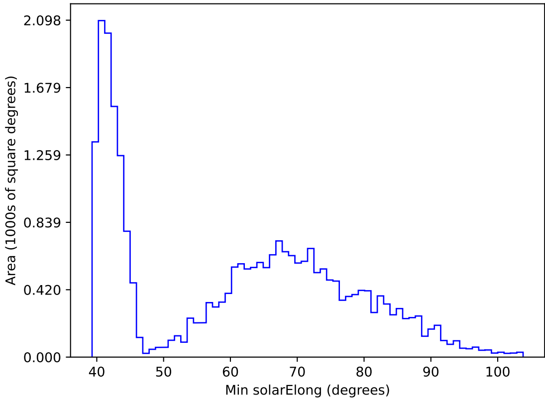
ddf_acor_sf20_ls40_lsr50_v3.4_10yrs All sky r band: Min solarElong
