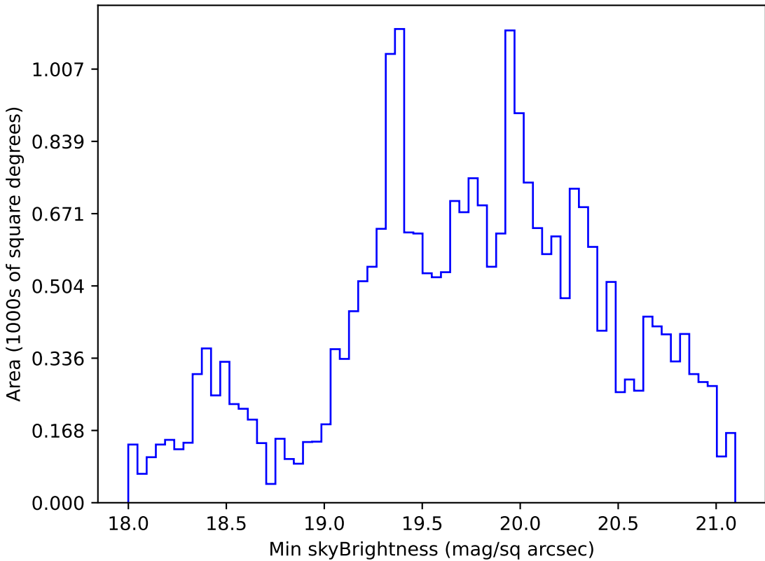
ddf_acor_sf20_lsf40_lsr50_v3.4_10yrs Yr 1 r band: Min skyBrightness
