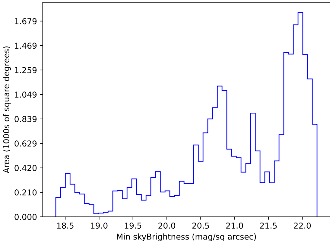
ddf_acor_sf20_lsf40_lsr50_v3.4_10yrs Yr 1 g band: Min skyBrightness
