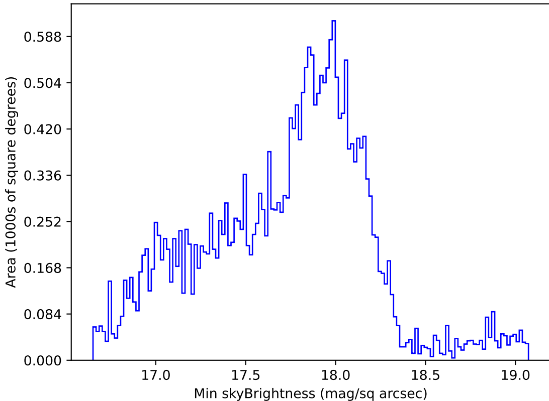
ddf_acor_sf20_lsf40_lsr50_v3.4_10yrs Yr 1 all bands: Min skyBrightness
