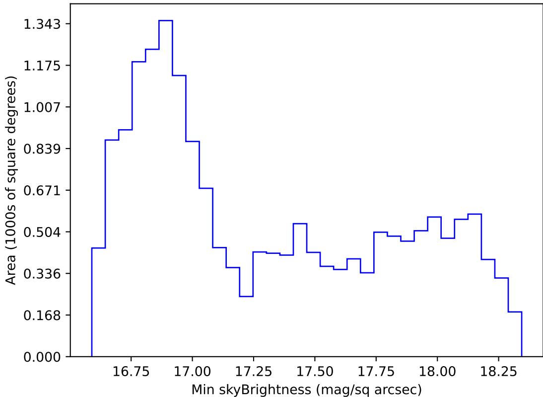
ddf_acor_sf20_lsf40_lsr50_v3.4_10yrs WFD z band: Min skyBrightness
