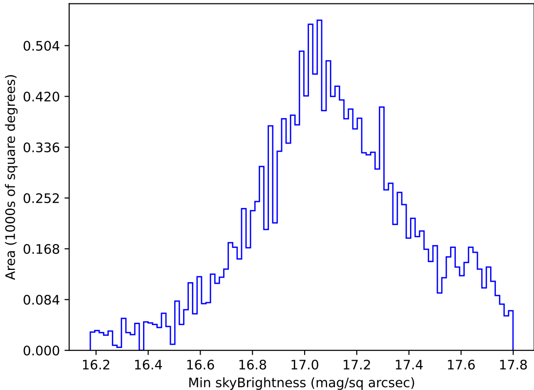
ddf_acor_sf20_lsf40_lsr50_v3.4_10yrs WFD y band: Min skyBrightness
