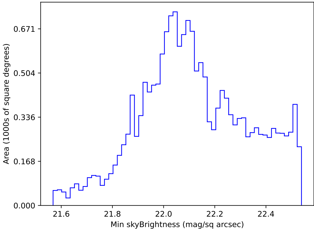
ddf_acor_sf20_lsf40_lsr50_v3.4_10yrs WFD u band: Min skyBrightness
