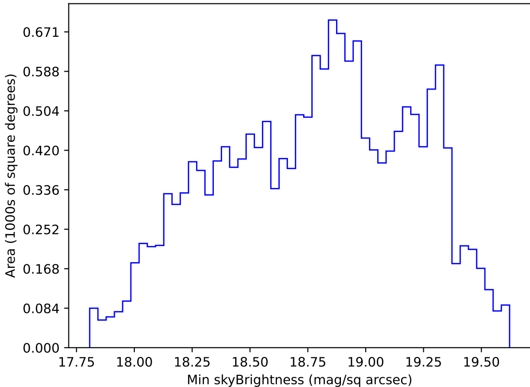
ddf_acor_sf20_lsf40_lsr50_v3.4_10yrs WFD r band: Min skyBrightness
