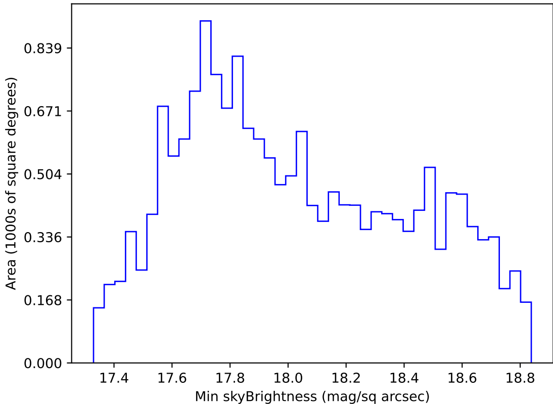
ddf_acor_sf20_lsf40_lsr50_v3.4_10yrs WFD i band: Min skyBrightness
