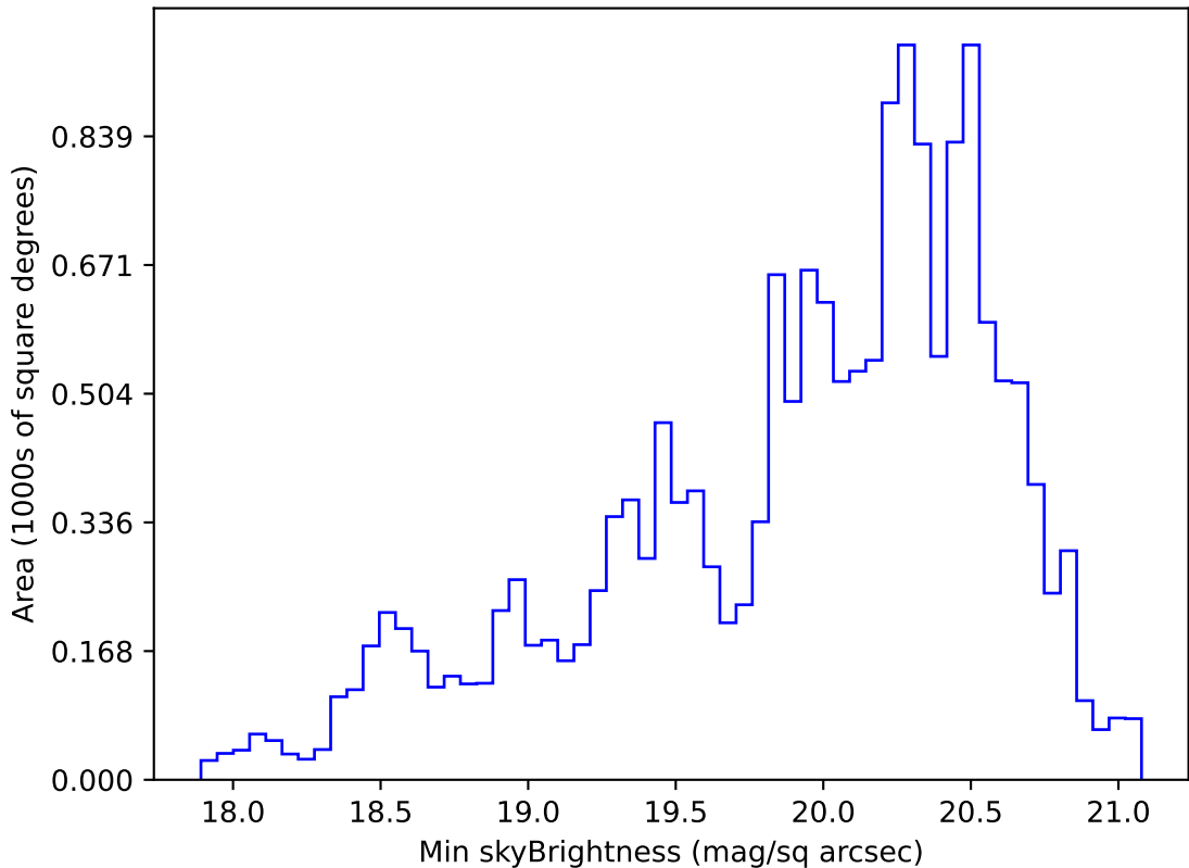
ddf_acor_sf20_lsf40_lsr50_v3.4_10yrs WFD g band: Min skyBrightness
