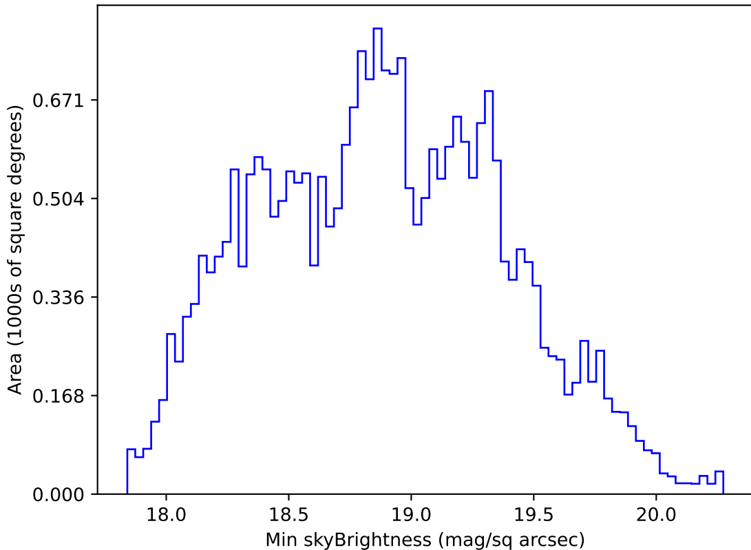
ddf_acor_sf20_lsf40_lsr50_v3.4_10yrs All sky r band: Min skyBrightness
