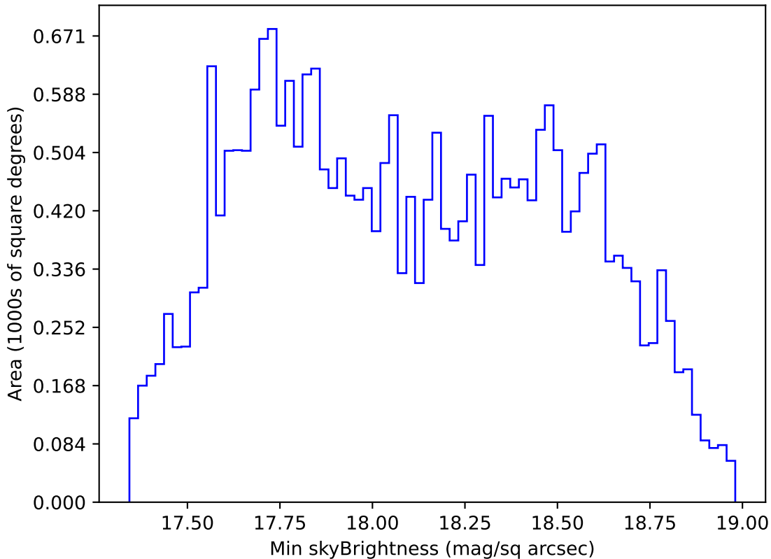
ddf_acor_sf20_lsf40_lsr50_v3.4_10yrs All sky i band: Min skyBrightness
