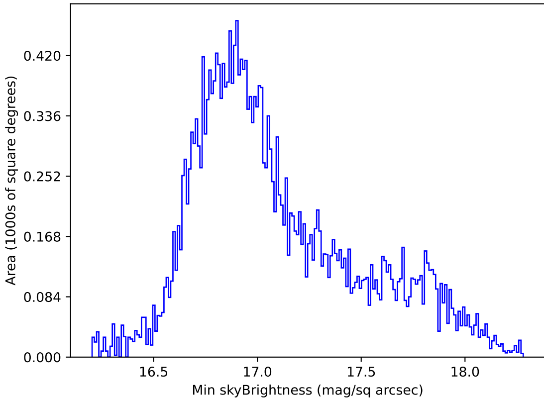
ddf_acor_sf20_lsf40_lsr50_v3.4_10yrs All sky all bands: Min skyBrightness
