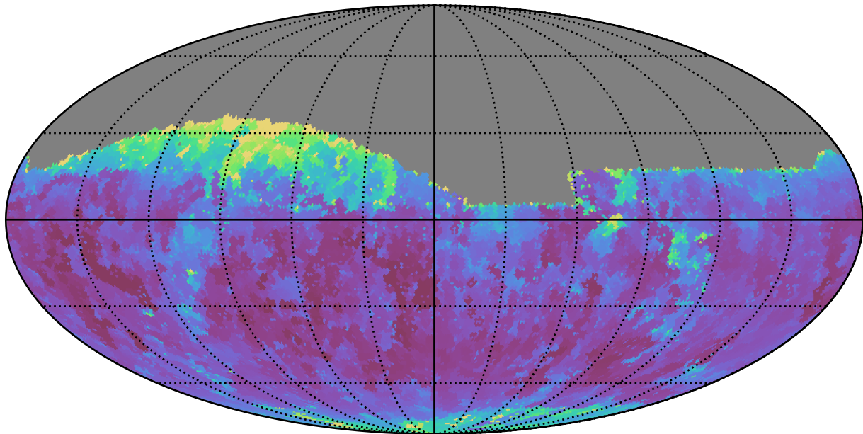
ddf_acor_sf20_lsf40_lsr50_v3.4_10yrs Yr 1 z band: Min seeingEff
