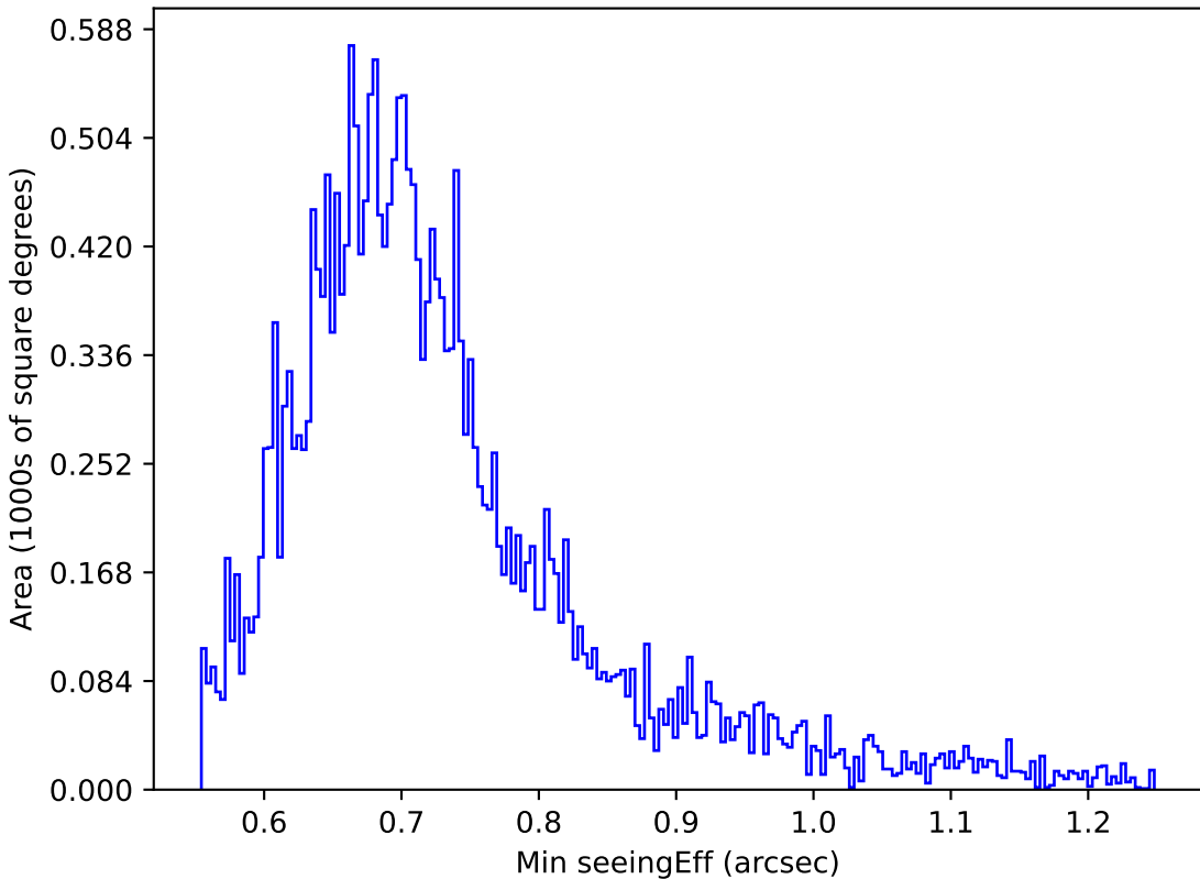
ddf_acor_sf20_ls40_lsr50_v3.4_10yrs Yr 1 z band: Min seeingEff
