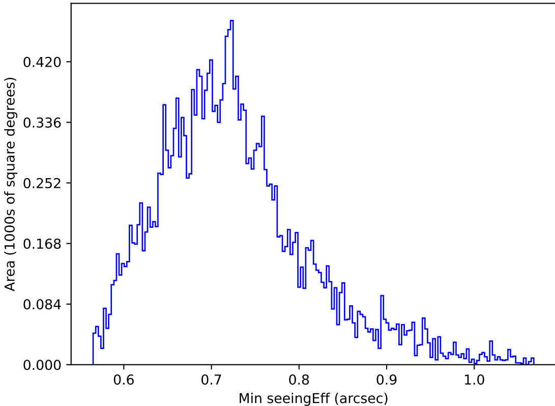
ddf_acor_sf20_ls40_lsr50_v3.4_10yrs Yr 1 y band: Min seeingEff
