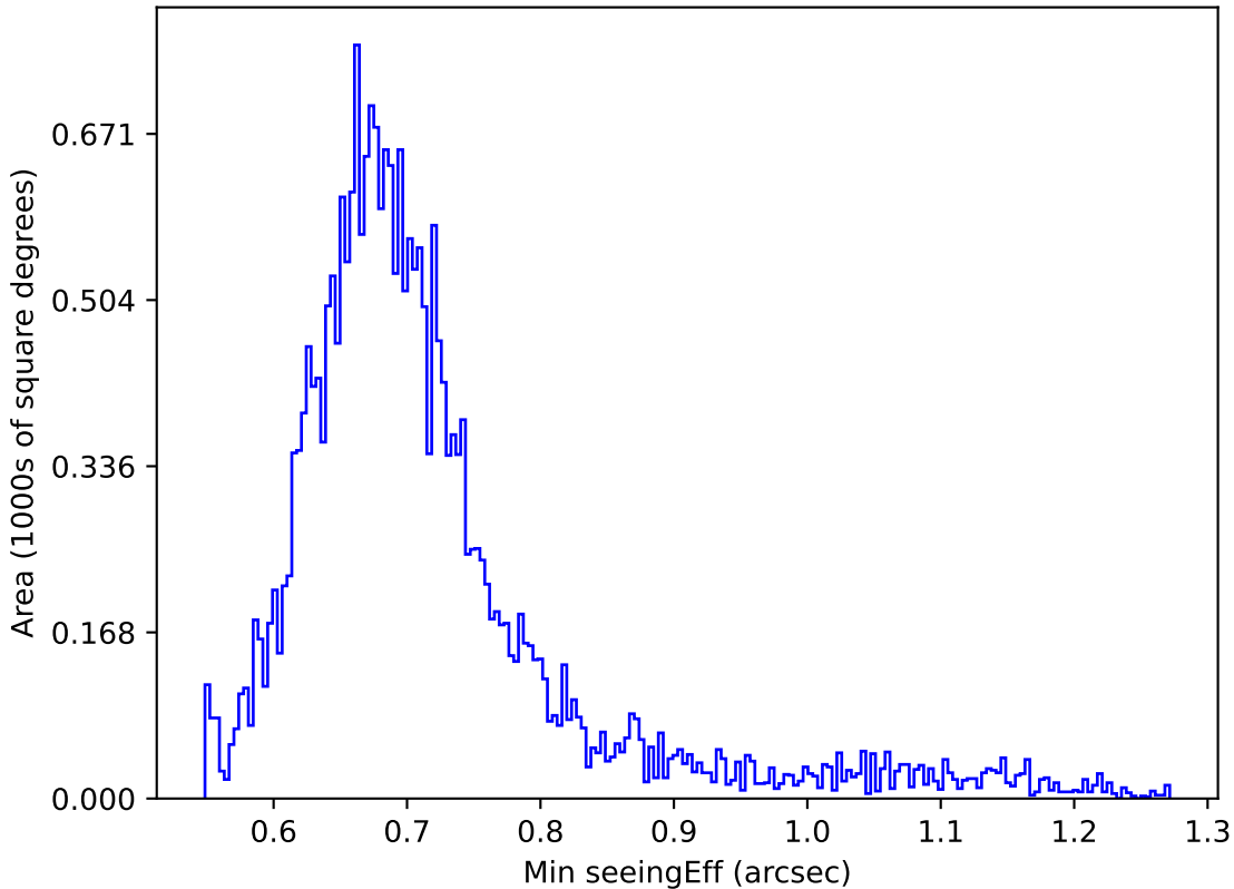
ddf_acor_sf20_ls40_lsr50_v3.4_10yrs Yr 1 r band: Min seeingEff
