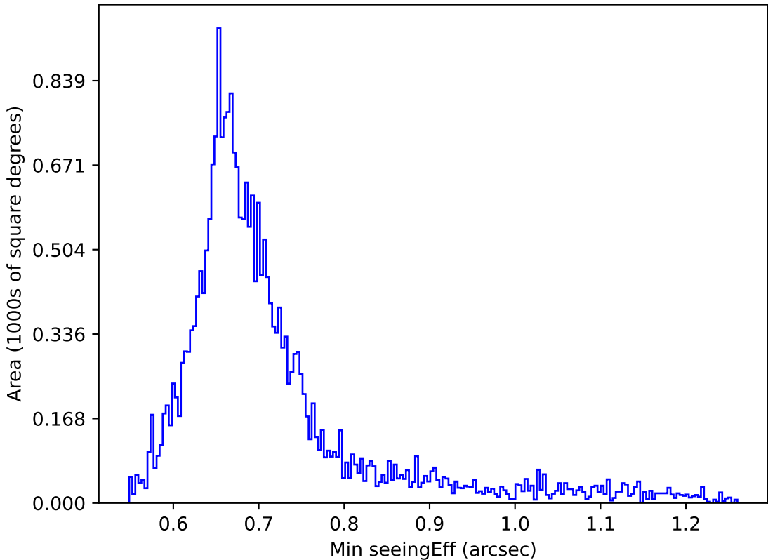
ddf_acor_sf20_lsf40_lsr50_v3.4_10yrs Yr 1 i band: Min seeingEff
