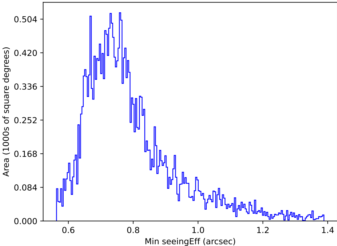
ddf_acor_sf20_lsf40_lsr50_v3.4_10yrs Yr 1 g band: Min seeingEff
