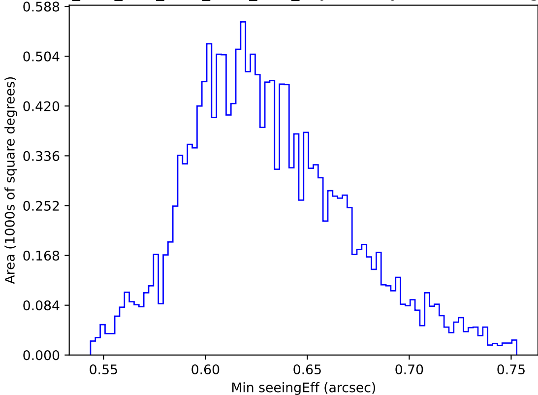
ddf_acor_sf20_lsf40_lsr50_v3.4_10yrs WFD y band: Min seeingEff
