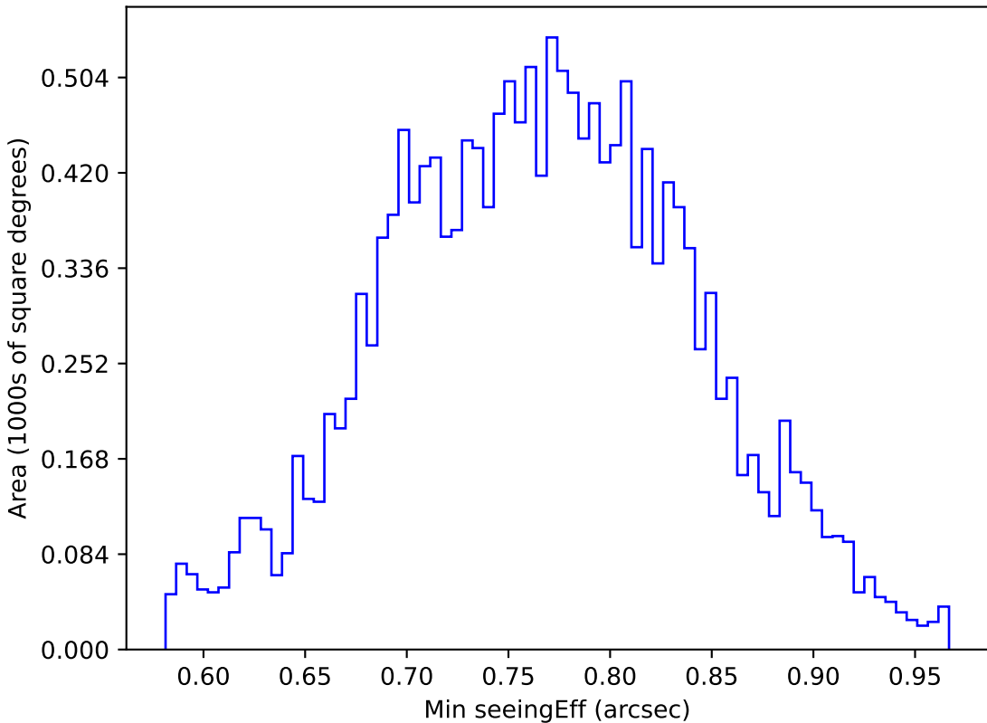
ddf_acor_sf20_lsf40_lsr50_v3.4_10yrs WFD u band: Min seeingEff
