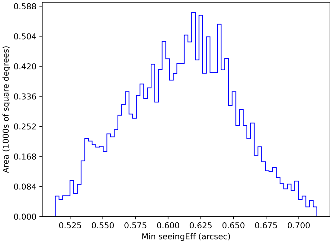
ddf_acor_sf20_lsf40_lsr50_v3.4_10yrs WFD r band: Min seeingEff
