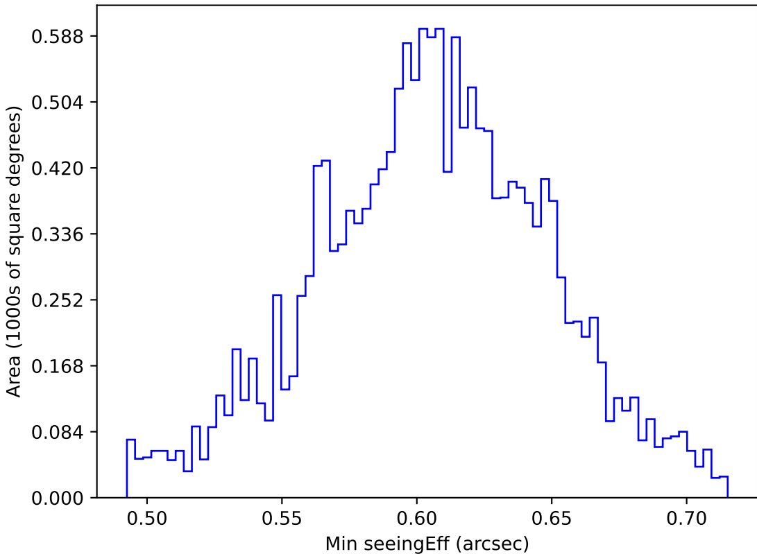
ddf_acor_sf20_lsf40_lsr50_v3.4_10yrs WFD i band: Min seeingEff
