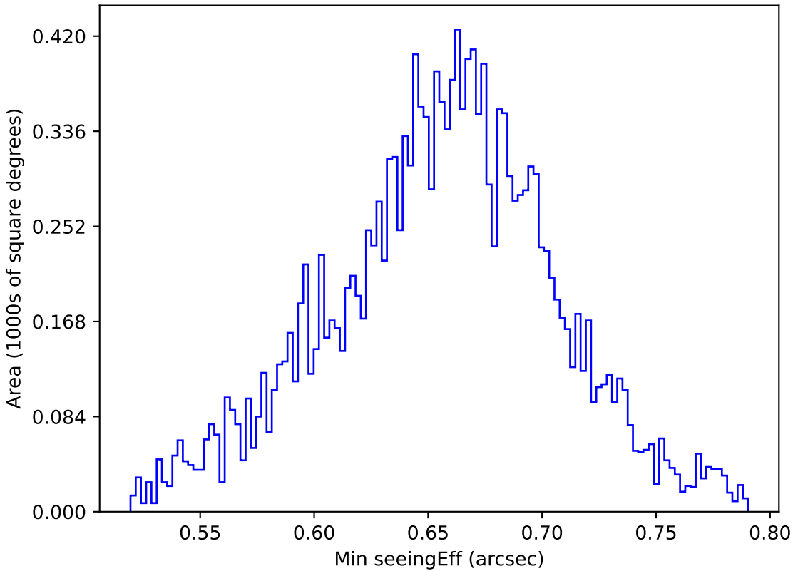
ddf_acor_sf20_lsf40_lsr50_v3.4_10yrs WFD g band: Min seeingEff
