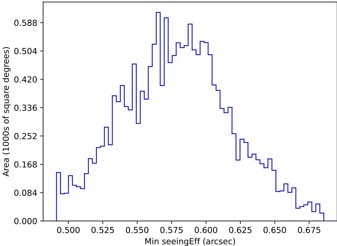
ddf_acor_sf20_lsf40_lsr50_v3.4_10yrs WFD all bands: Min seeingEff
