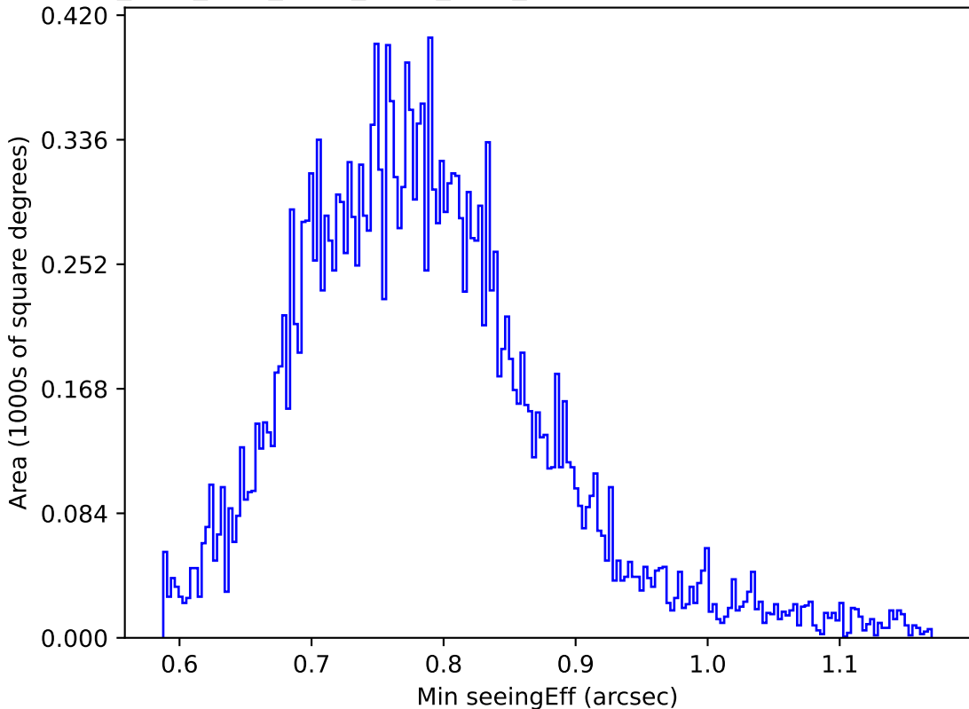
ddf_acor_sf20_lsf40_lsr50_v3.4_10yrs All sky u band: Min seeingEff
