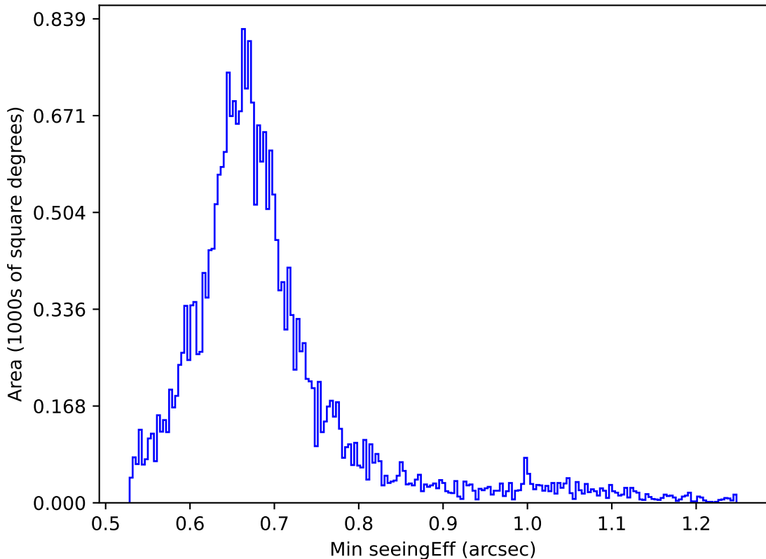
ddf_acor_sf20_lsf40_lsr50_v3.4_10yrs All sky g band: Min seeingEff
