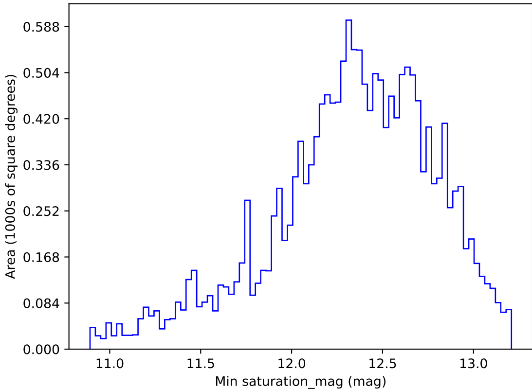
ddf_acor_sf20_lsf40_lsr50_v3.4_10yrs WFD i band: Min saturation_mag
