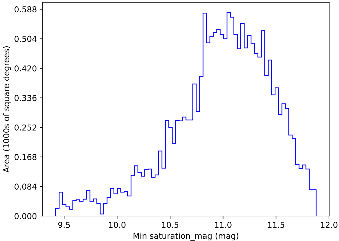
ddf_acor_sf20_lsf40_lsr50_v3.4_10yrs WFD all bands: Min saturation_mag
