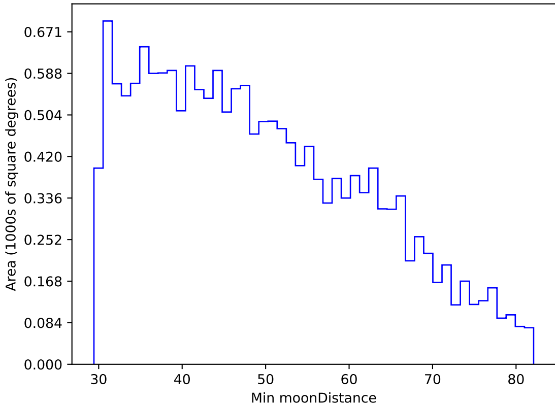
ddf_acor_sf20_lsf40_lsr50_v3.4_10yrs WFD u band: Min moonDistance
