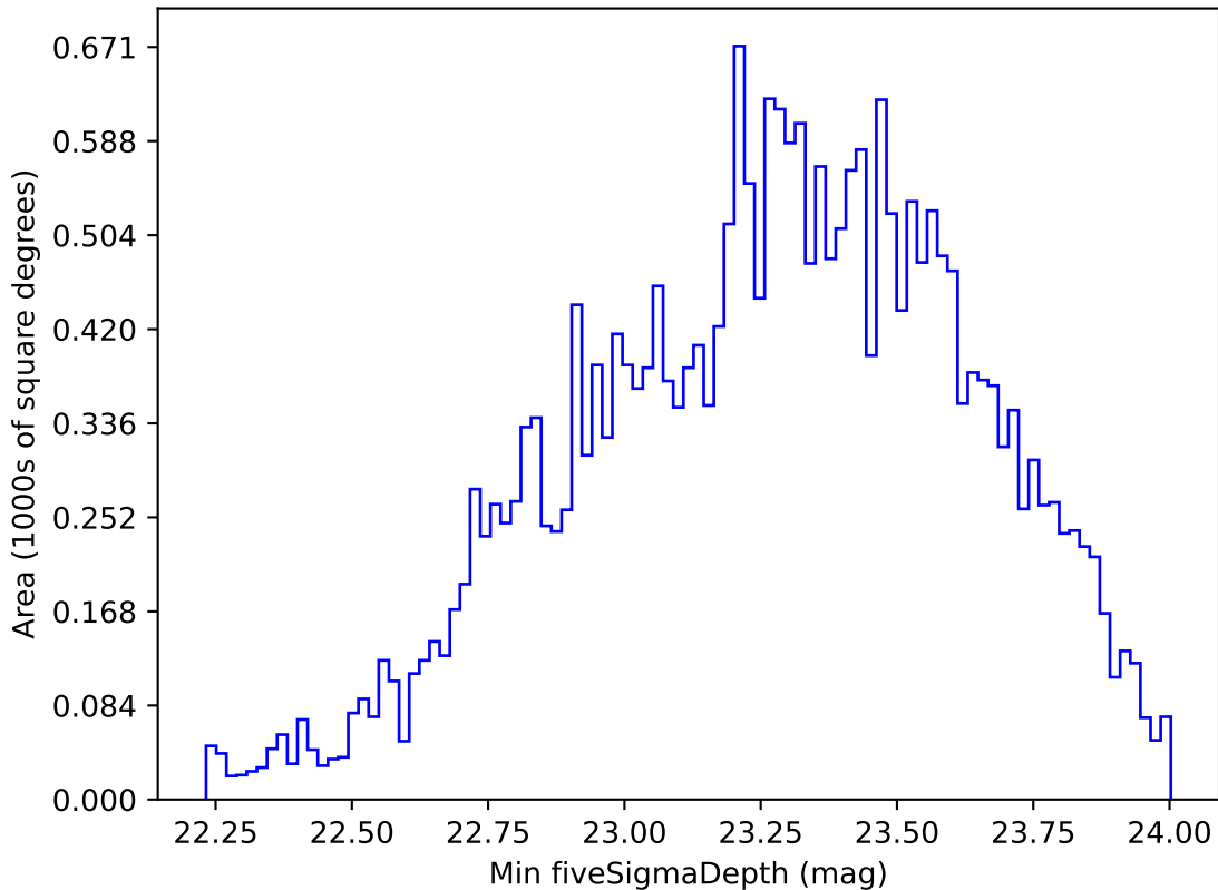
ddf_acor_sf20_lsf40_lsr50_v3.4_10yrs All sky g band: Min fiveSigmaDepth
