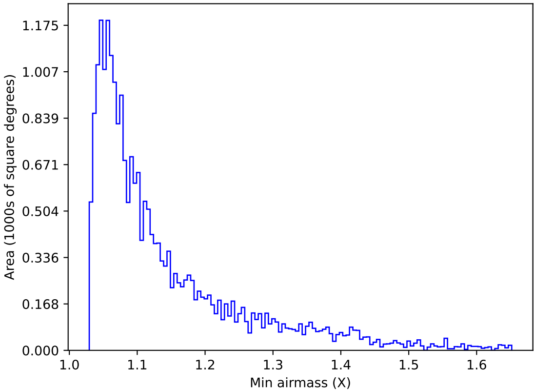
ddf_acor_sf20_lsf40_lsr50_v3.4_10yrs Yr 1 u band: Min airmass
