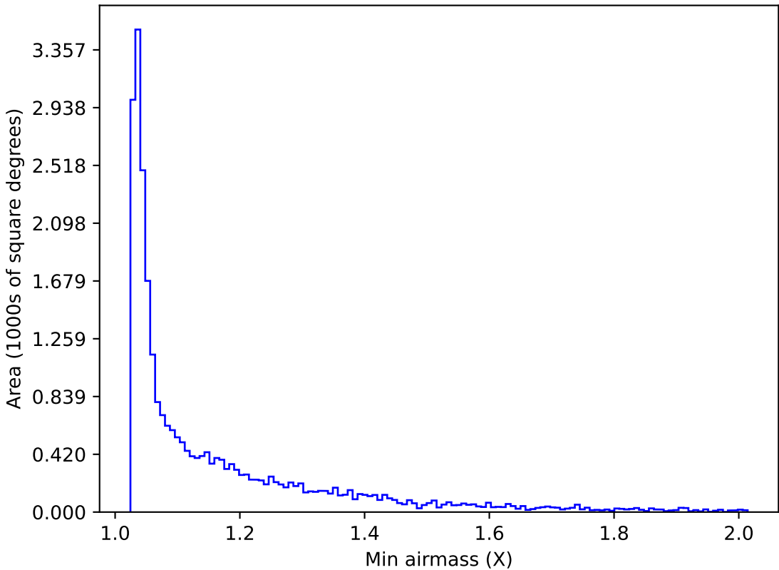
ddf_acor_sf20_lsf40_lsr50_v3.4_10yrs Yr 1 i band: Min airmass
