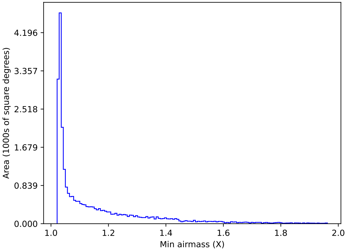
ddf_acor_sf20_lsf40_lsr50_v3.4_10yrs Yr 1 all bands: Min airmass
