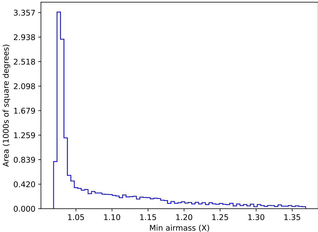
ddf_acor_sf20_lsf40_lsr50_v3.4_10yrs WFD z band: Min airmass
