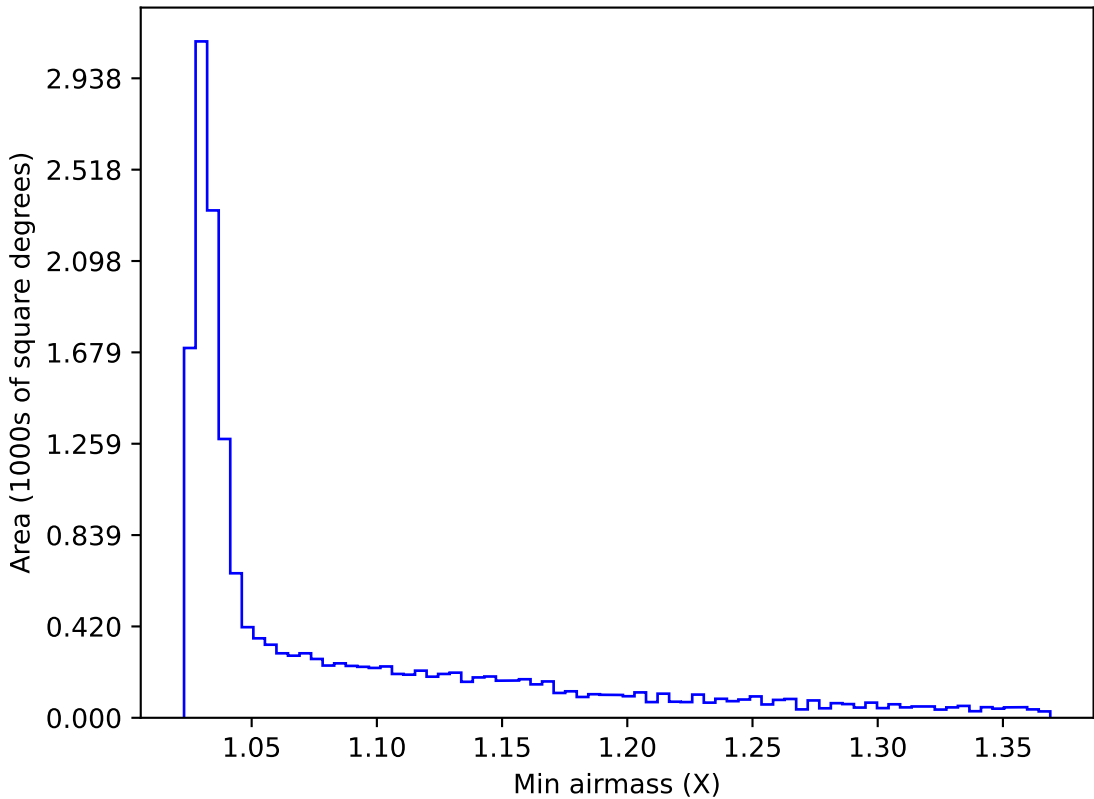
ddf_acor_sf20_lsf40_lsr50_v3.4_10yrs WFD y band: Min airmass
