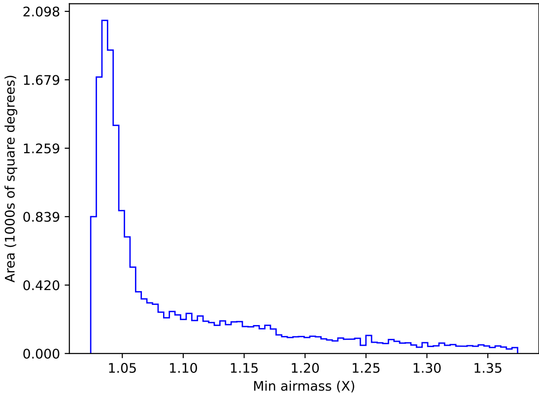
ddf_acor_sf20_lsf40_lsr50_v3.4_10yrs WFD u band: Min airmass
